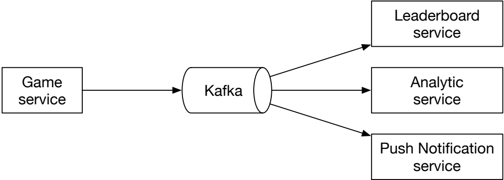
Figure 4 Game scores are used by multiple services
